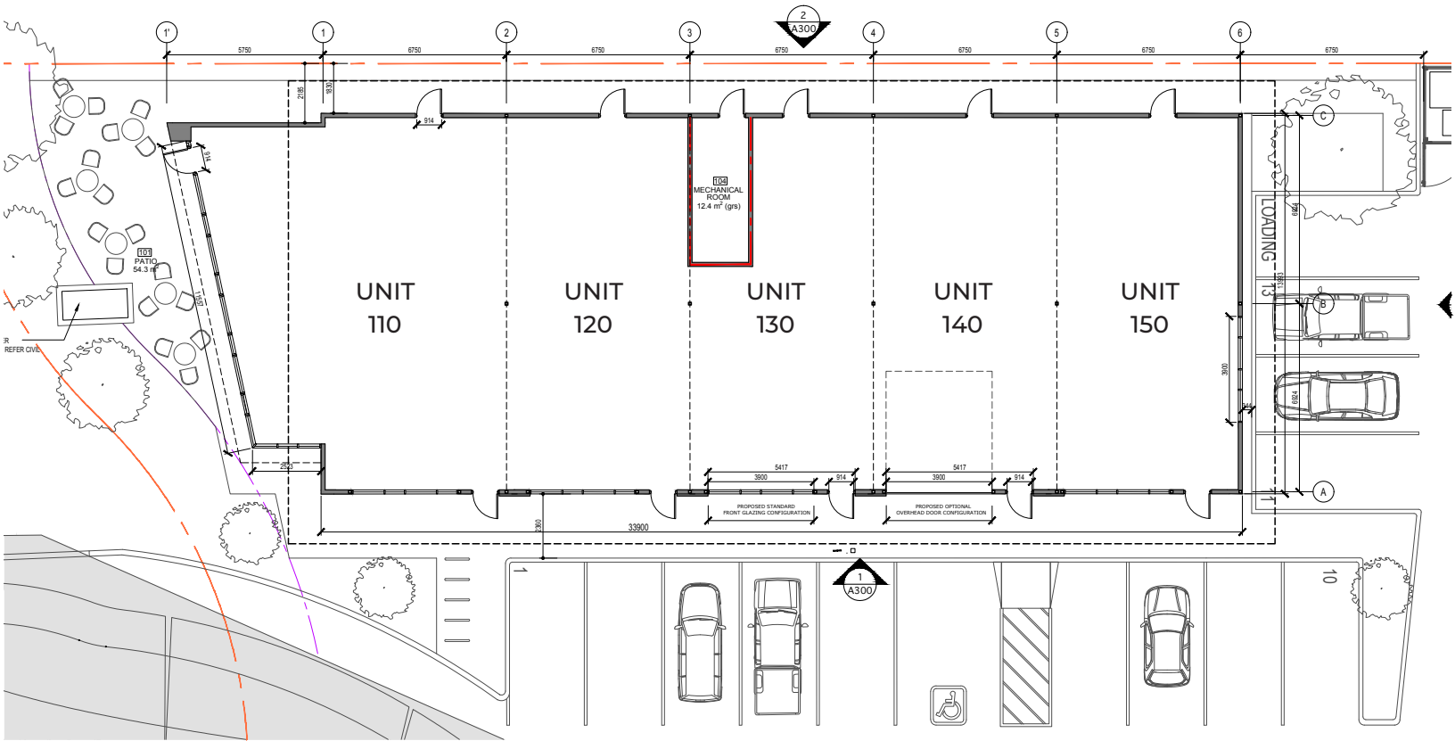
1 200 FLOOR PLAN 1:100
